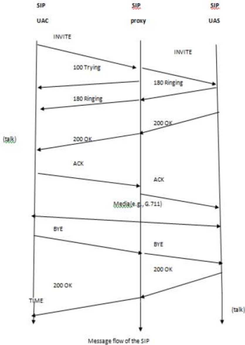
Fig.2. Message flow of the SIP
