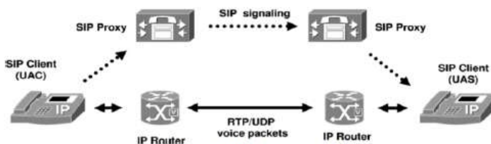
Fig. 1. SIP Trapezoid
