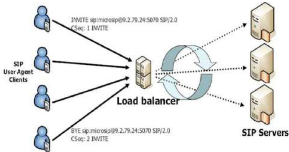
Fig. 3. System architecture
